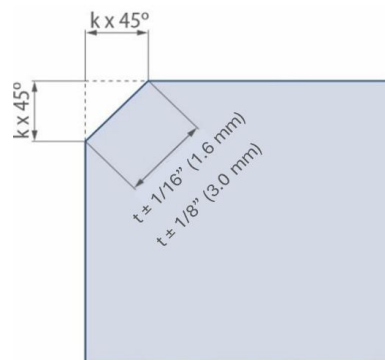
Fig. 16 Corner cut-off
