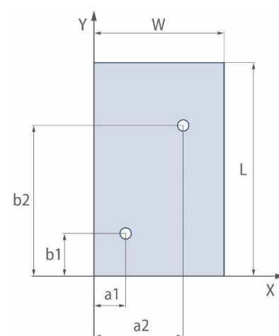
Fig. 13 Hole position
